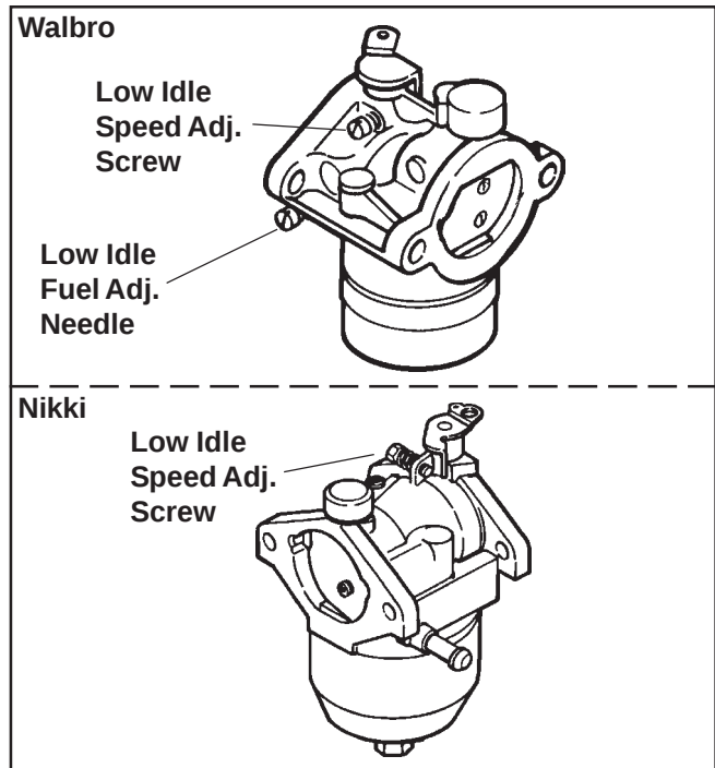
Figure 11. Carburetor.
