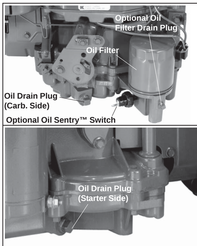
Figure 8. Oil Drain Plugs, Oil Filter, Oil Filter Drain Plug, and Optional Oil Sentry™ Switch.
