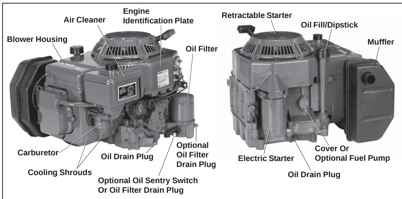
Figure 1. Typical Command Vertical Shaft Engine.
