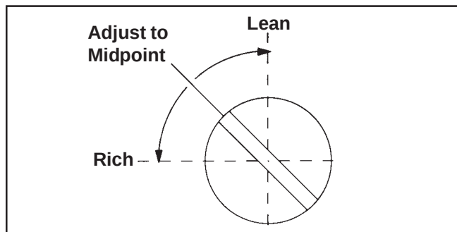
Figure 12. Optimum Low Idle Fuel Setting.
