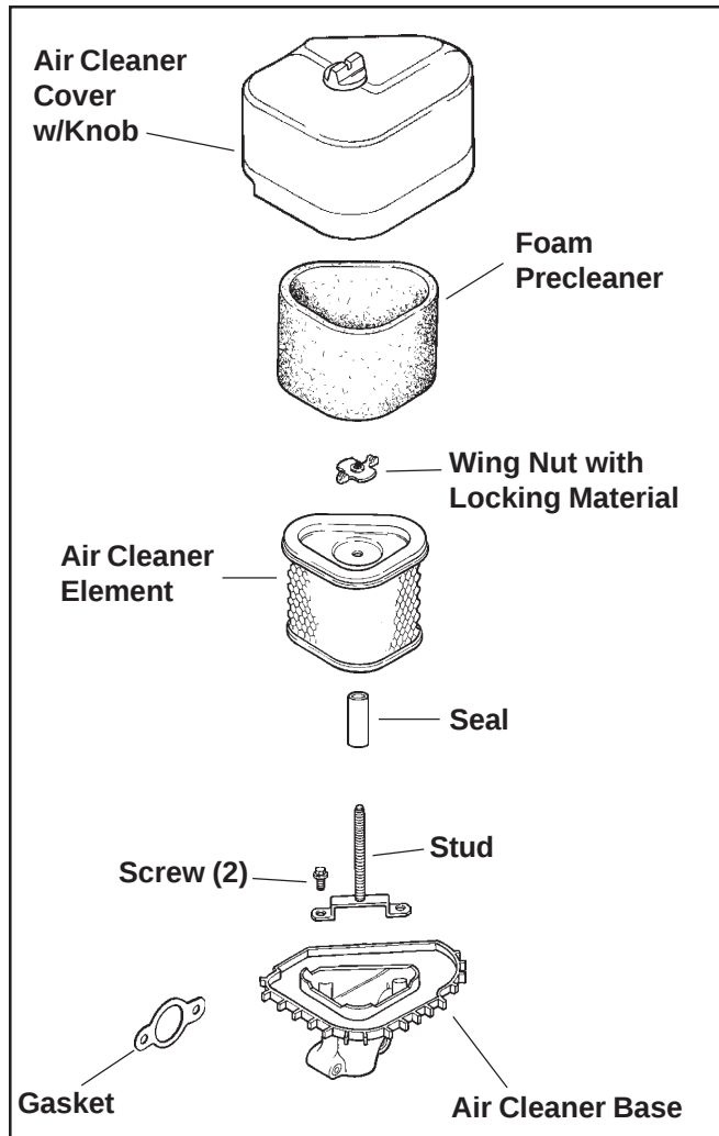
Figure 9. Air Cleaner Assembly – Exploded View.
